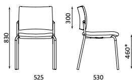
INTRATA V-31 FL NA weight: 6,60 kg
