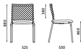
INTRATA V-32 FL NA weight: 6,70 kg
