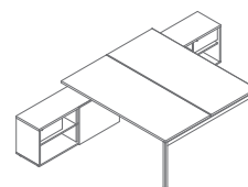
BOYL41 1800-1902 / 3210 / 740 210.4 kg
