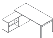
BOYL21 1800-1902 / 1600 / 740 106.75 kg
