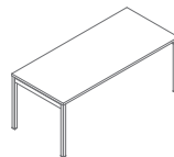
BOY05 1800 / 800 / 740 48.35 kg
