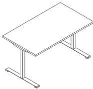
BOT54 1400 / 800 / 740 43.45 kg
