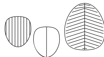
Alberi
